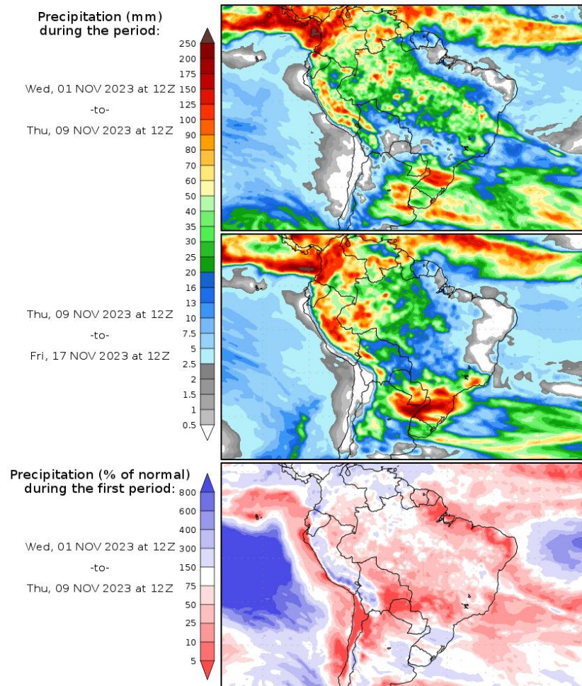
Precipitation Forecasts
