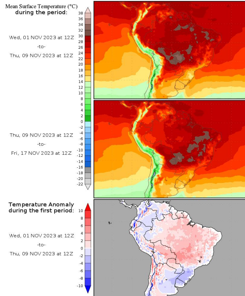
Temperature Forecasts
